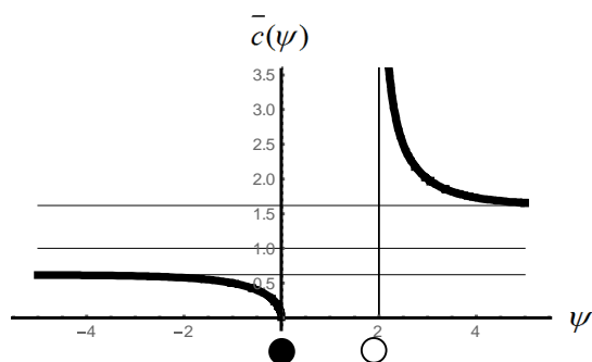
Fig. 2.1. The graph \bar{c}(\psi) > 0 for the case \{-\infty < \psi < 0\} \cup \{2 < \psi < +\infty\} (The black curve)
