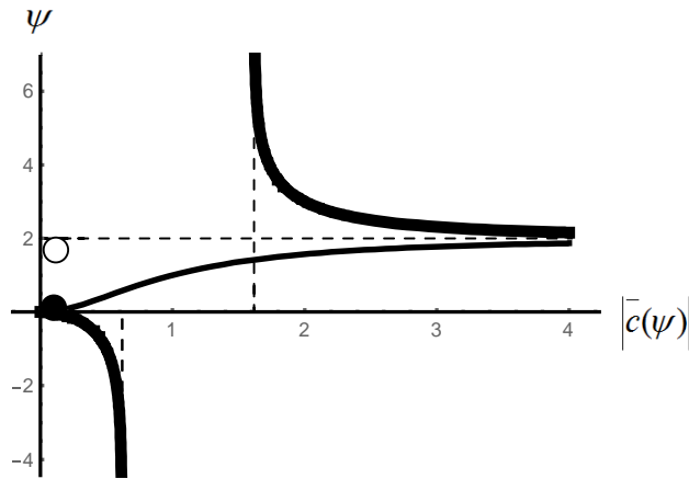
Fig. 3.2. The graph of the dependence of the parameter of self-organization \psi from the module |\bar{c}(\psi)| of the normalized Fibonacci light velocity in vacuum \bar{c}(\psi)
