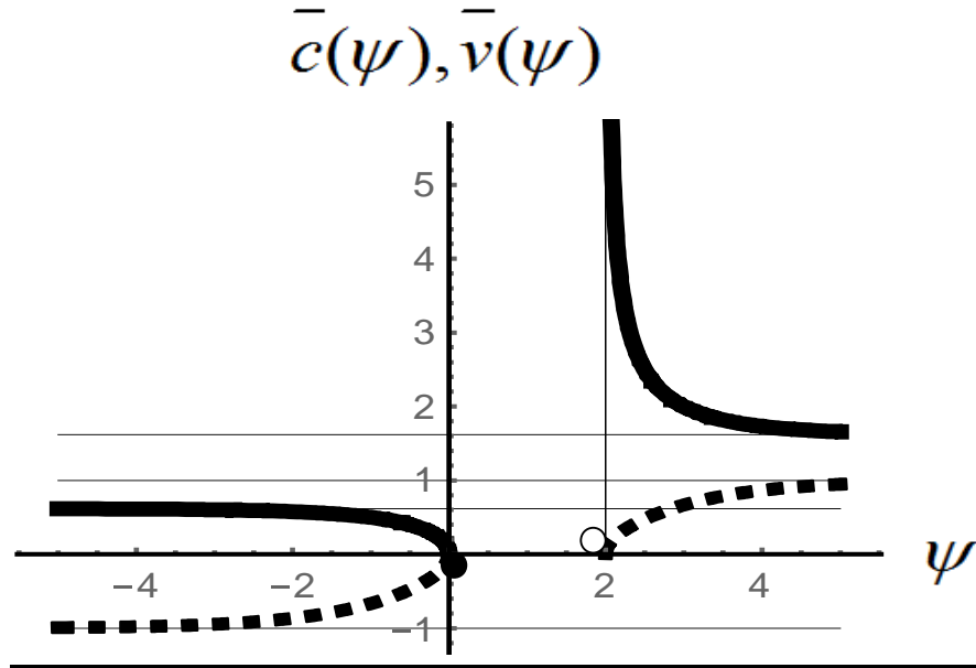
Fig. 2.2. The graph \bar{c}(\psi) (the black curves) and the graph \bar{v}(\psi) (the dashed curves), where the parameter \psi is in limits \{-\infty < \psi < 0\} \cup \{2 < \psi < +\infty\} . The symbols \bullet and \circ correspond to the bifurcation points \psi = 0 and \psi = 2 .
