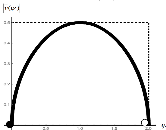
Fig. 2.4. The graph of the module |\bar{v}(\psi)| on the interval \{0 < \psi < 2\}
