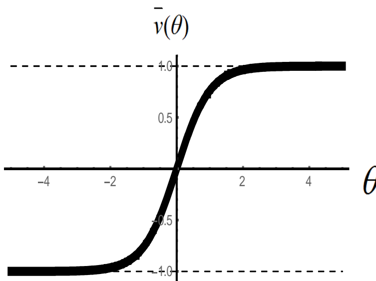
Fig. 1.1. The graph of the normalized speed of the light source \bar{v}(\theta) = \frac{v(\theta)}{c} = th(\theta) (the black curve), \lim_{\theta \rightarrow \pm\infty} \bar{v}(\theta) = \pm 1 are the limit values of the normalized speed of the light source (the dashed lines)
