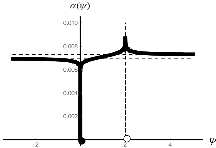
Fig. 3.1. The graph of the fine-structure constant (black curve) at \{-\infty < \psi < \infty\}
