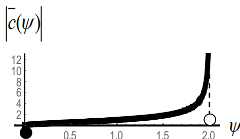
Fig. 2.3. The graph of the module |\bar{c}(\psi)| in the range \{0 < \psi < 2\}
